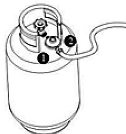
Leak Test Point ① ②
